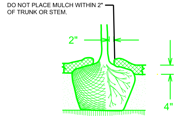
MULCH DETAIL
