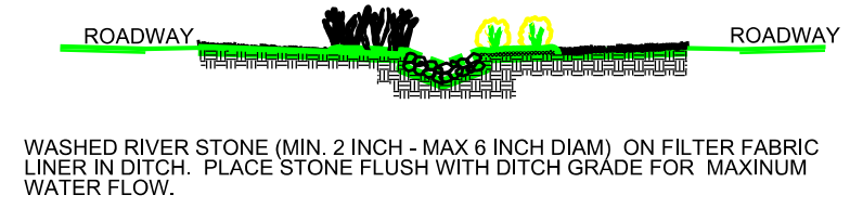
RIVERSTONE DITCH LINING DETAIL
