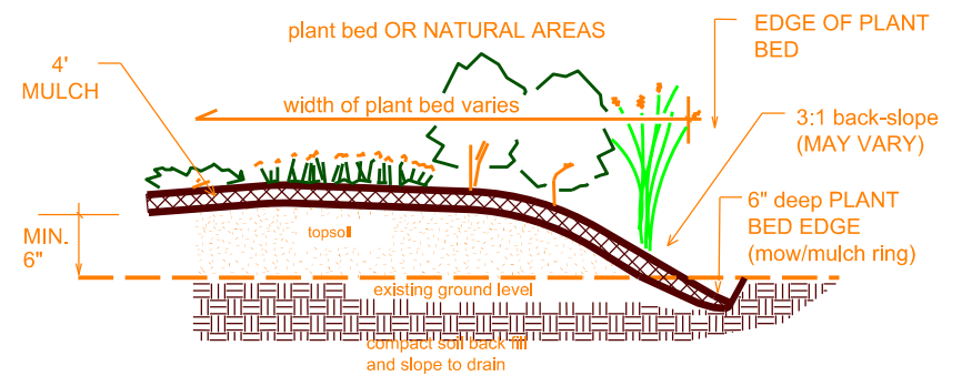
PLANT BED EDGE DETAIL
